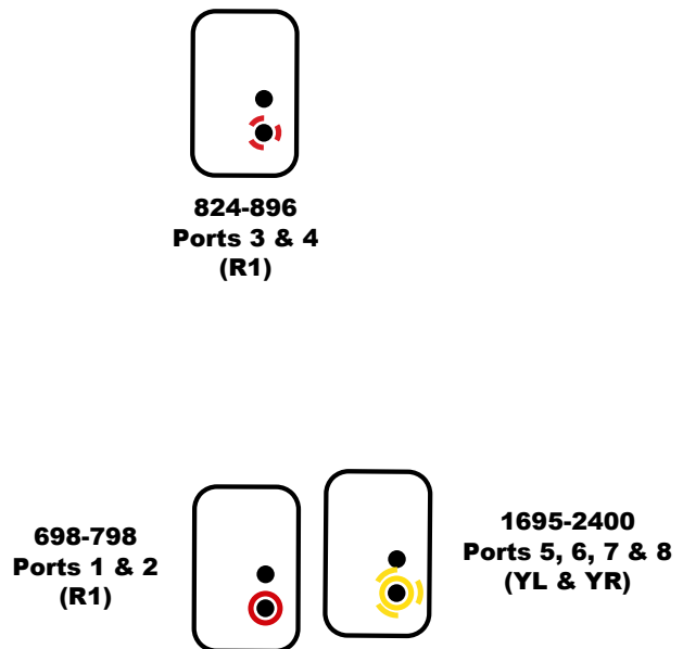
Top of antenna
