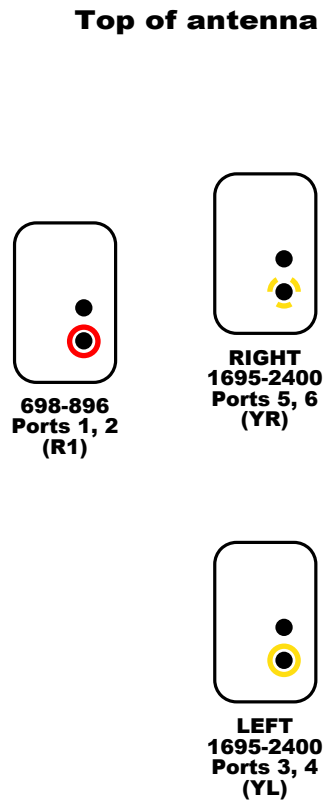
RET placement as view from rear of antenna
