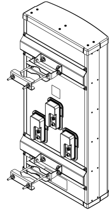
Fig. 3: Fixed Mast Brackets Attached To The Antenna
