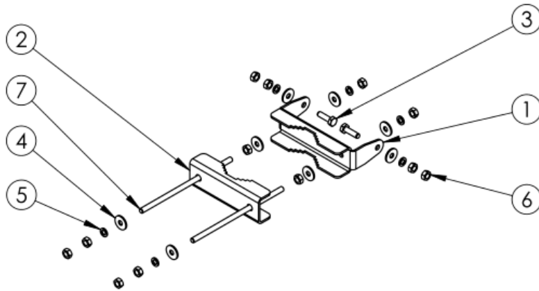
Fig. 1: Fixed Mast Bracket Kit BOM
