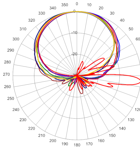
1720 MHz Azimuth with Elevation 5°
