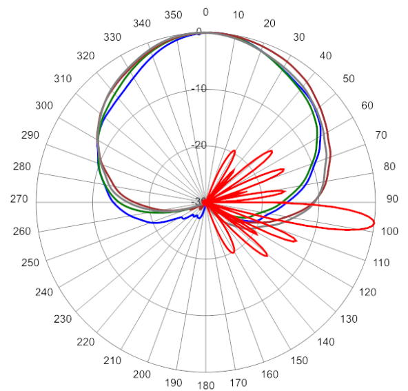
945 MHz Azimuth with Elevation 7°
