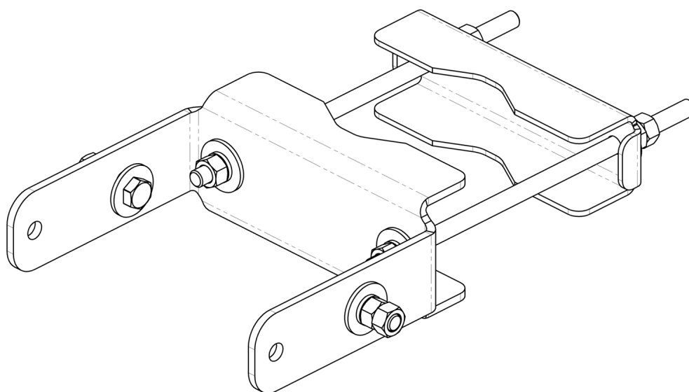
MBK-36 Top Bracket
