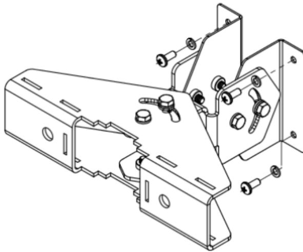
MBK-08 Adjustable Brackets
