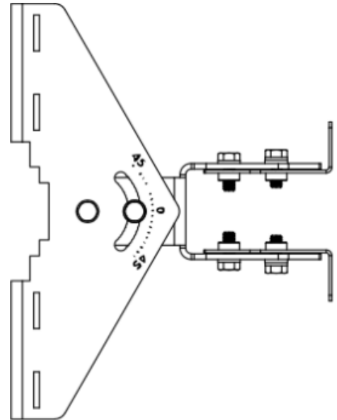
MBK-08 Adjustable Brackets Top View
