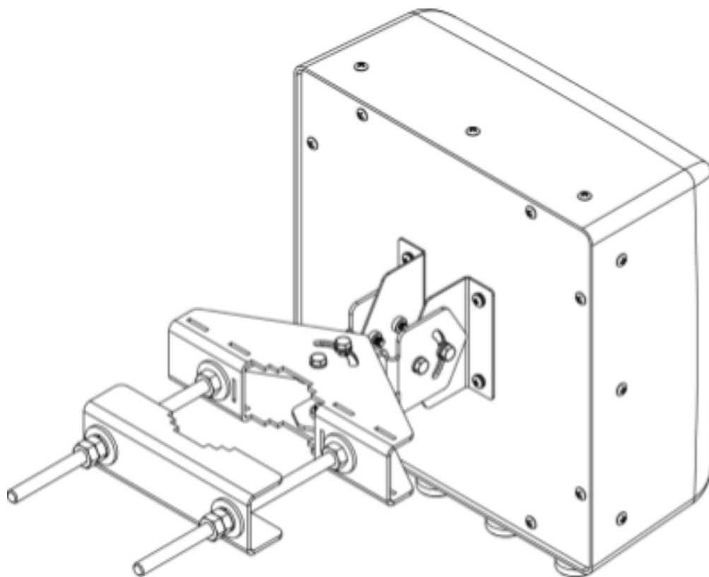
MBC-07 mounted to MBK-08
