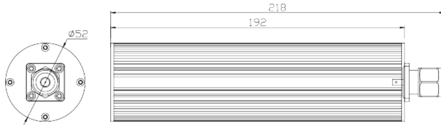
Ultra-broadband High Power Load with Male 4.3-10 Connector Outline Drawing bracket not shown
