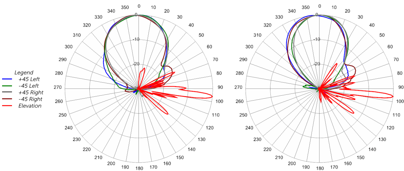
2155 MHz Azimuth with Elevation 6°
