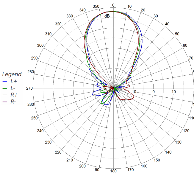
1948 MHz Azimuth
