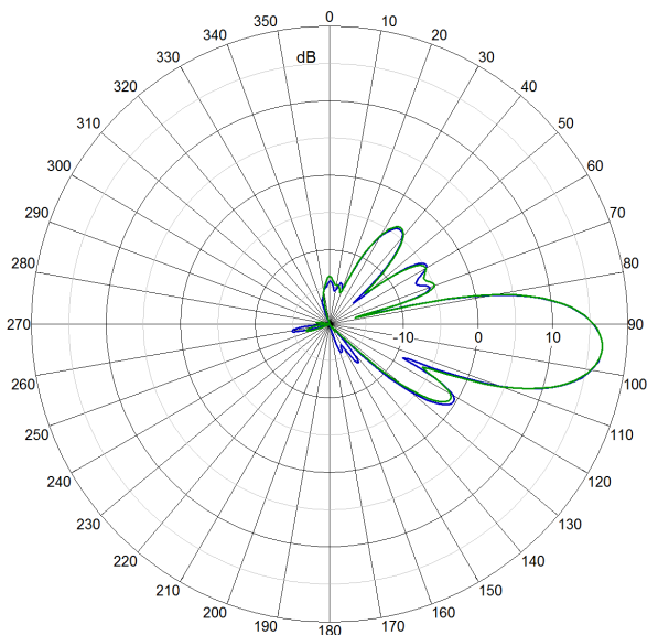
875 MHz Elevation 6°
