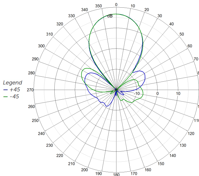
875 MHz Azimuth
