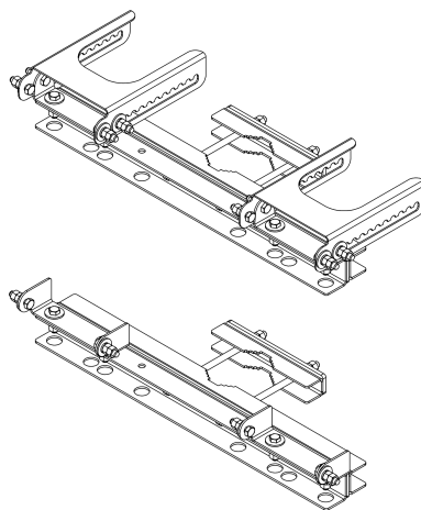
DM-01 Bracket
