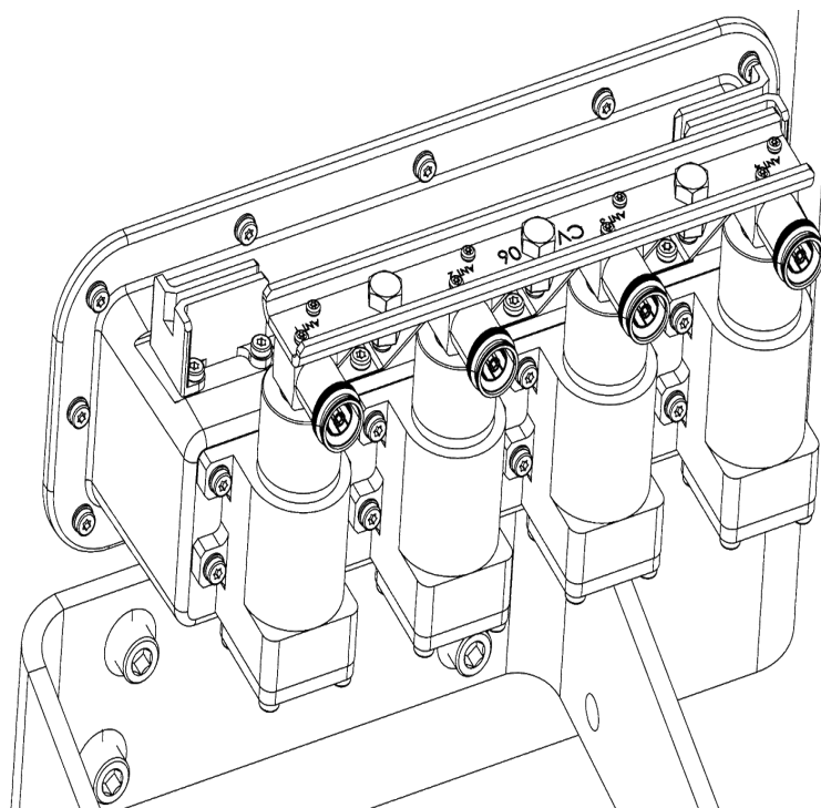
CV-06 installed onto Antenna
