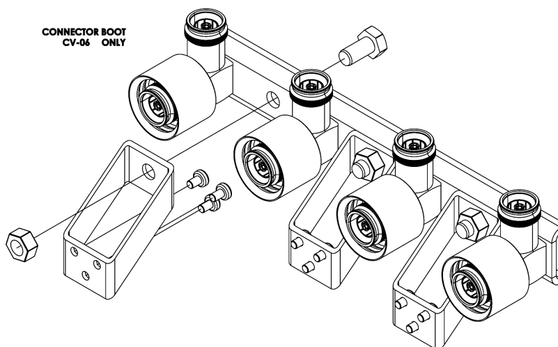
CV-06 Parts
