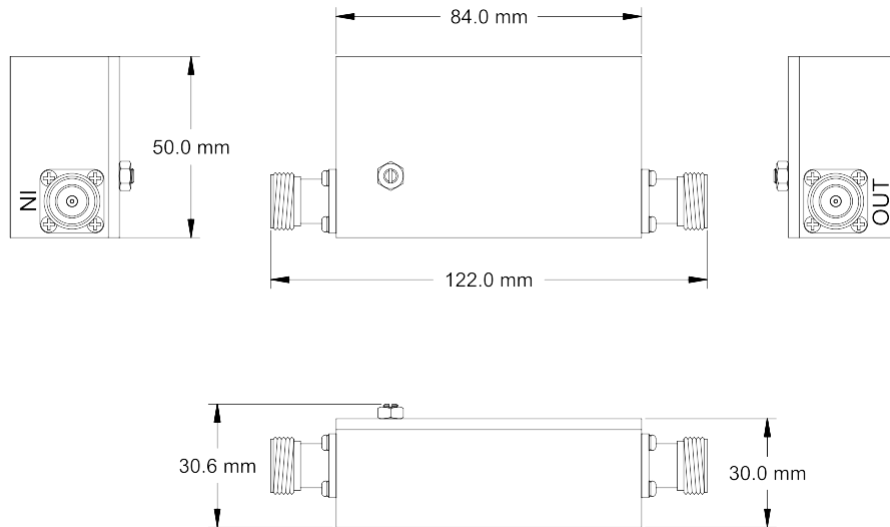
Indoor Passband Filter Outline Drawing BPT-1710785-0-S3
