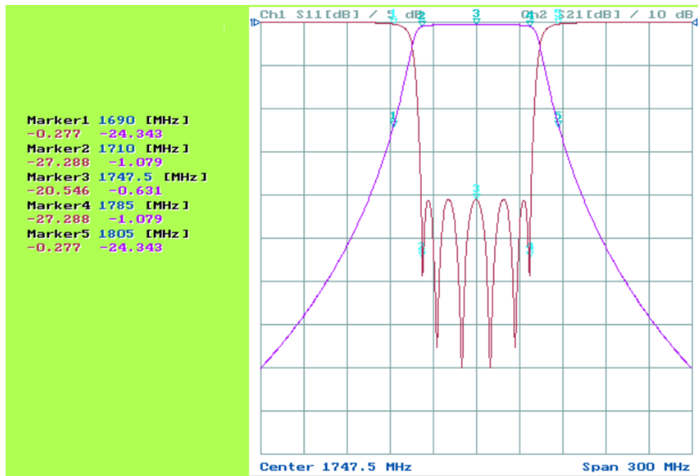
BPT-1710785-0-S3 RX Filter Characteristics
