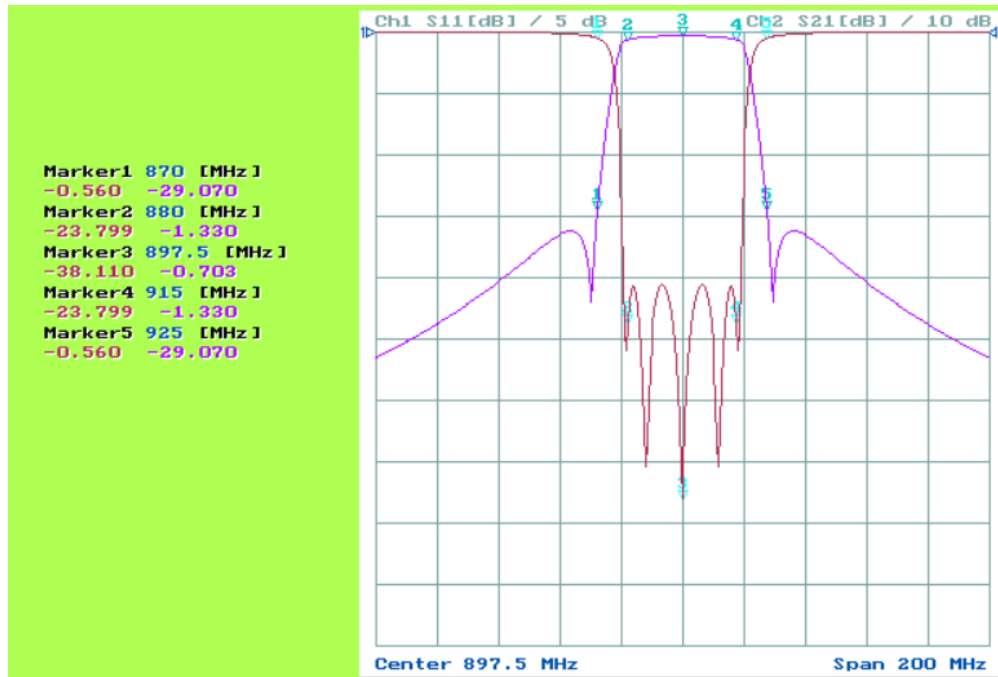
BPT-0880915-0-S3 RX Filter Characteristics
