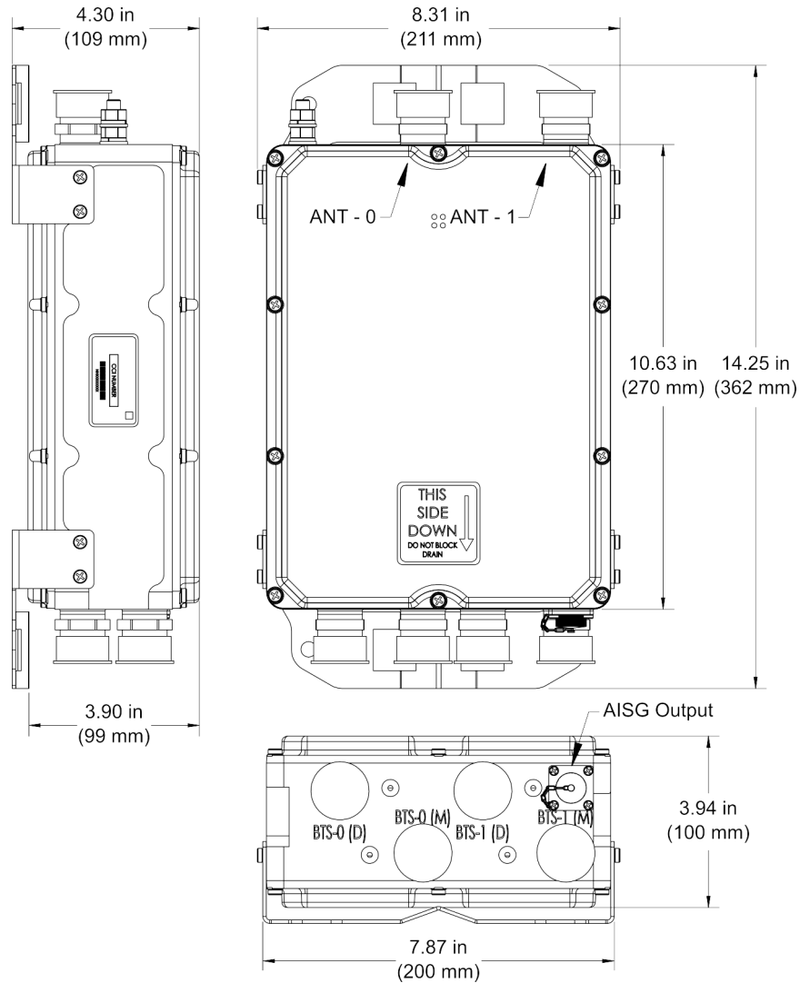
ASC1800VG10A Outline Drawing
