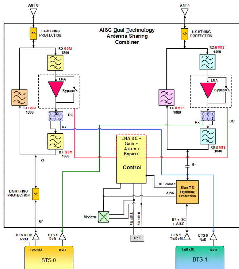
ASC1800VG10A Block Diagram
